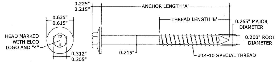
1 HEX FLANGE HEAD (HFH) 1'-0" = 1'-0"
